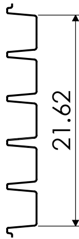
SECTION B-B
