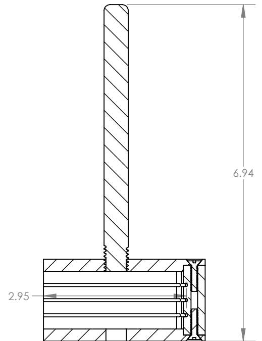
SECTION VIEW
